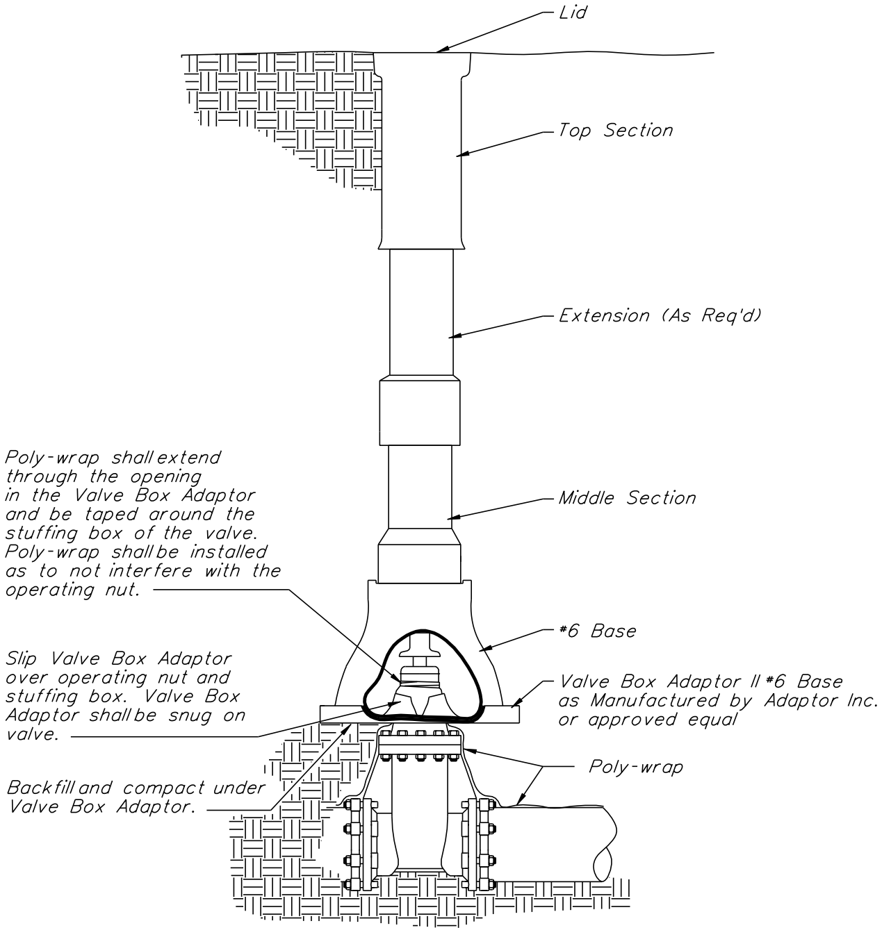
TYPICAL VALVE BOX (CC BOX) INSTALLATION
